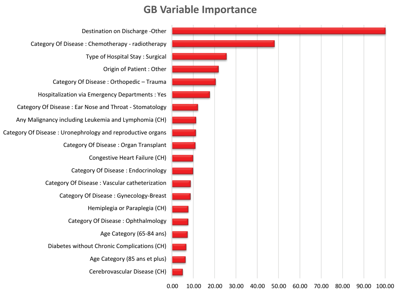
Figure 2. Gradient boosting variable importance (20 highest).
